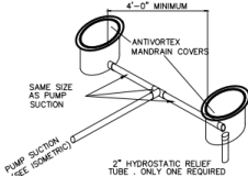
POOL MAINDRAIN DETAIL NO SCALE
