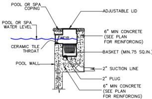
SKIMMER DETAIL NO SCALE
