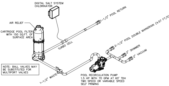
ISOMETRIC
